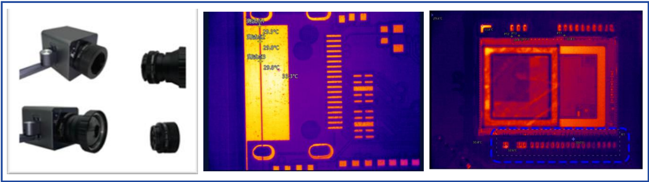
Study chip and electronic component's temperature change under macro lens
